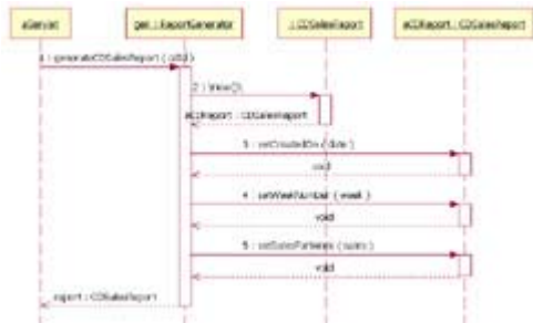
Figure 4: A sample sequence diagram ( click here to enlarge )
