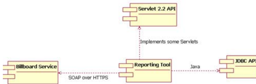
Figure 7: A component diagram shows interdependencies of various software components the system comprises
